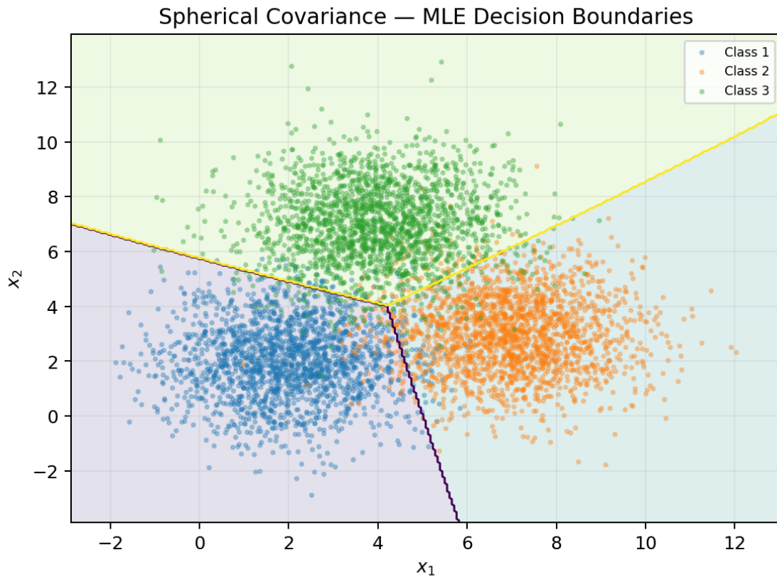
Figure: Spherical Covariance MLE decision boundaries with the 20% test data overlaid.
