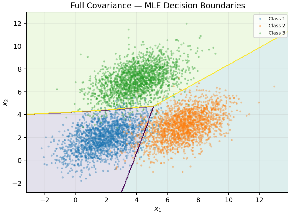
Figure: Full Covariance MLE decision boundaries with the 20% test data overlaid.
