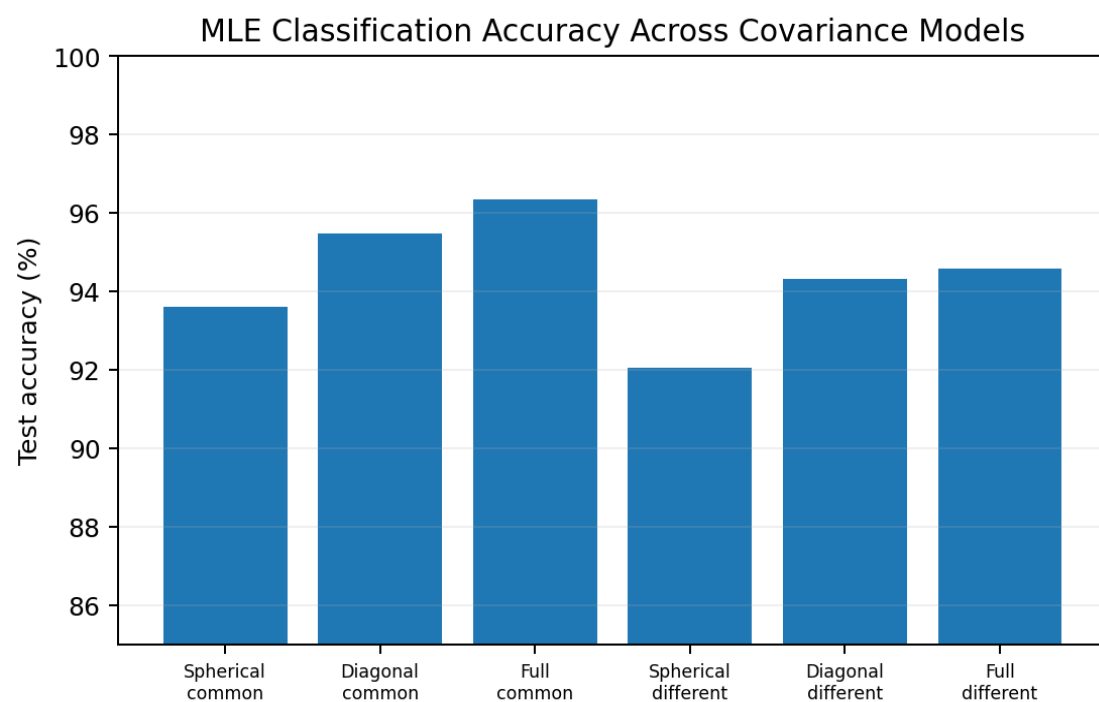
Figure: Comparison of MLE classification accuracy for the six covariance configurations.
