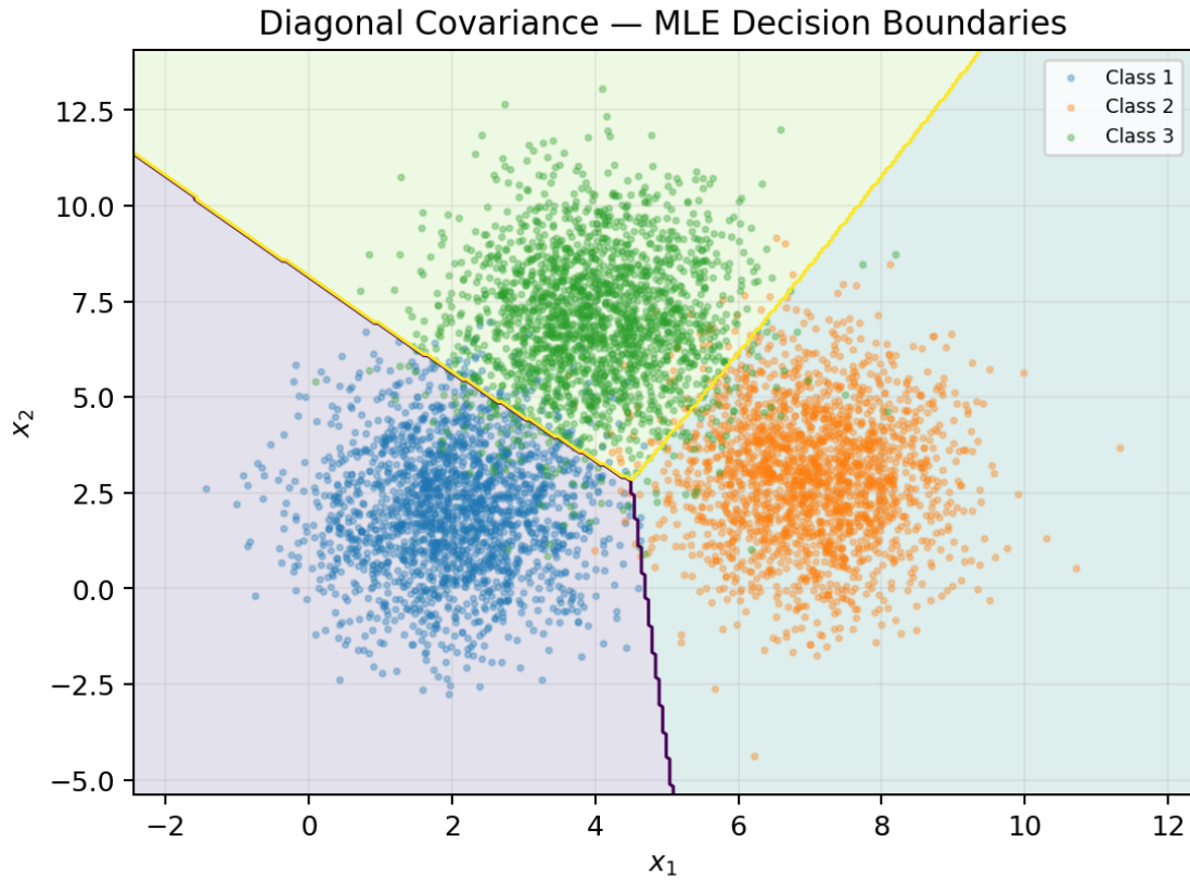
Figure: Diagonal Covariance MLE decision boundaries with the 20% test data overlaid.
