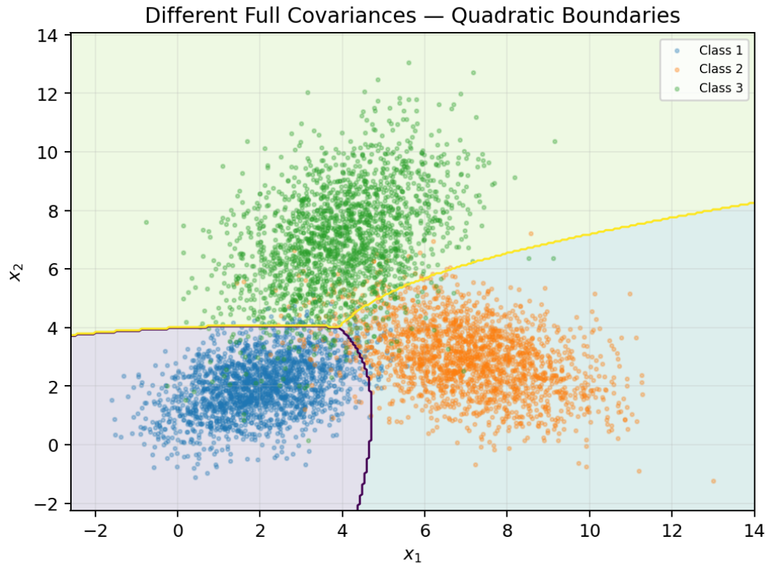
Figure: Full covariance with different class-specific covariance matrices. The test data are overlaid on the quadratic decision regions.
