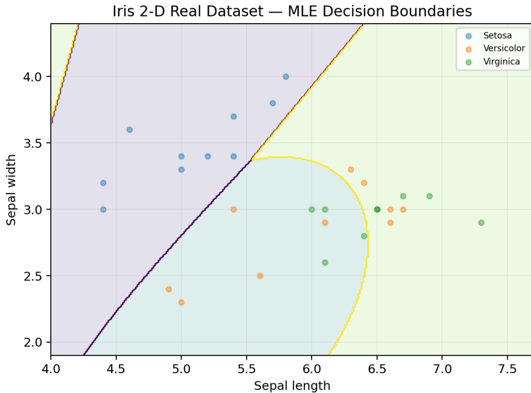
Figure: MLE decision boundaries for the real 2-D Iris dataset with the 20% test samples overlaid.
